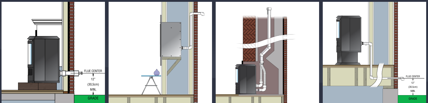
Zero-Clearance Fireplace Package
